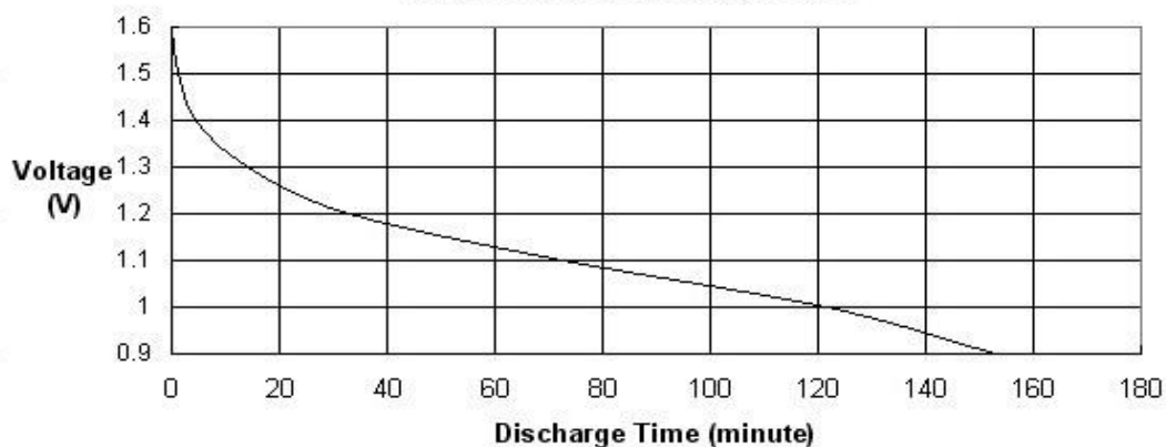
3.9 \Omega Continuous Discharge Curve
