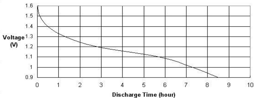
10 \Omega Continuous Discharge Curve
