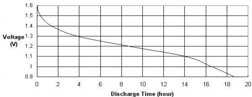
20 \Omega Continuous Discharge Curve
