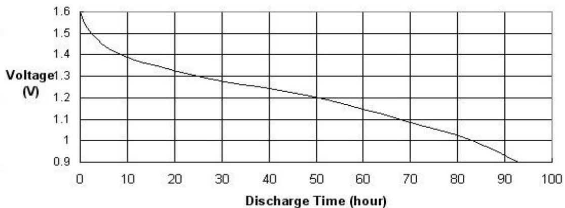
43 \Omega 4hour/day Discharge Curve
