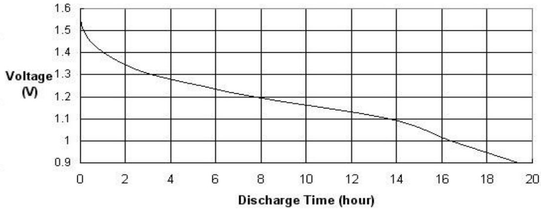
10 \Omega Continuous Discharge Curve
