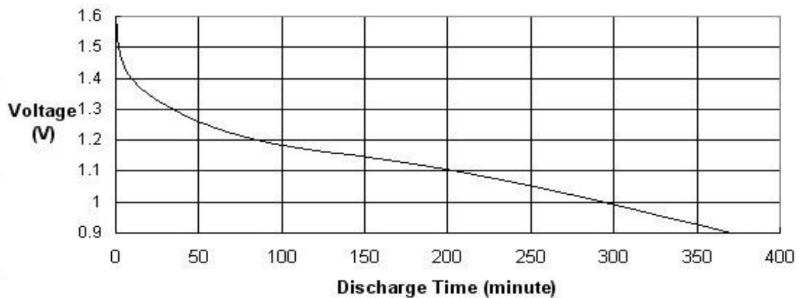
3.9 \Omega Continuous Discharge Curve
